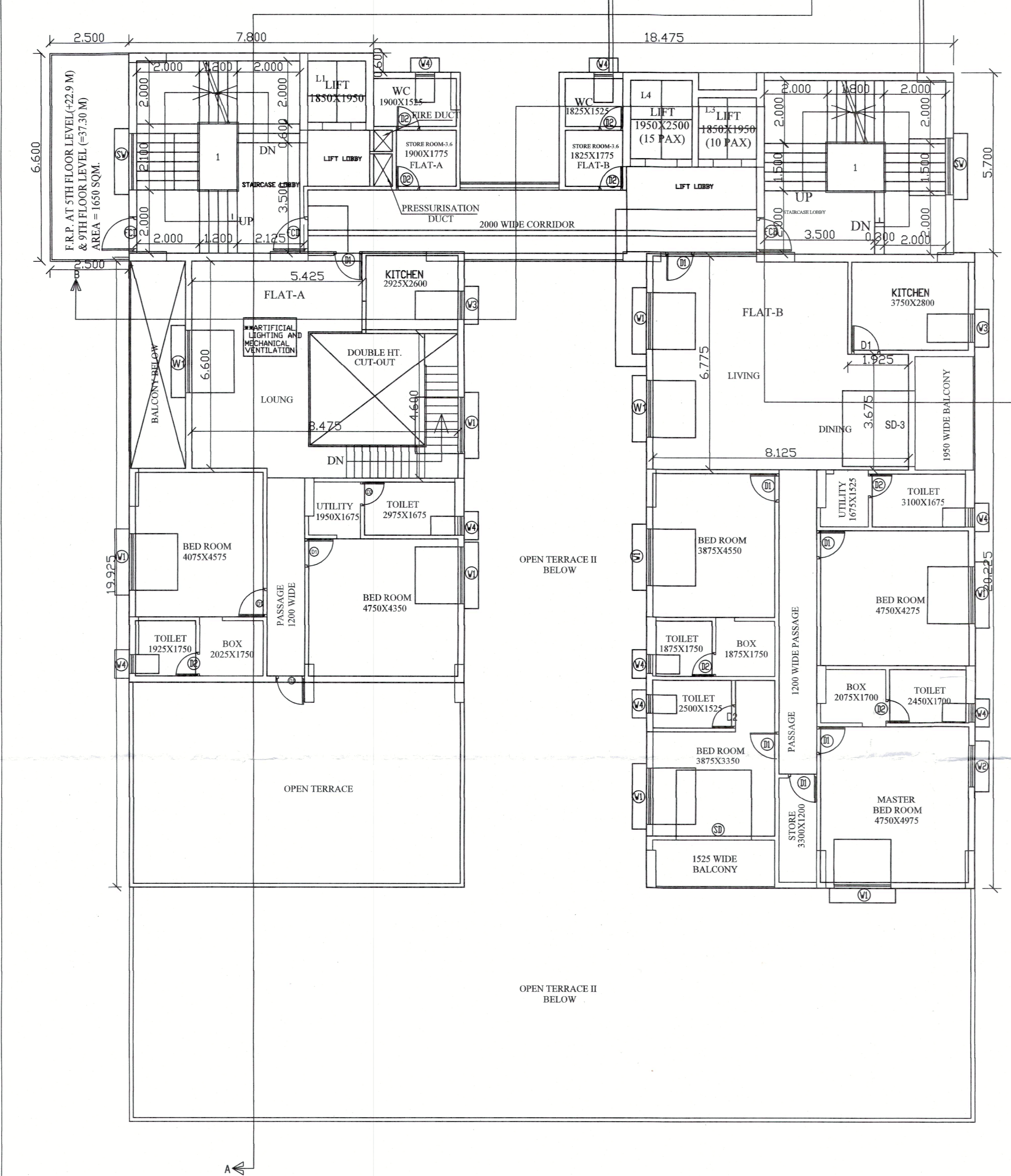
FLOOR 10 SCALE - 1:1 WING-1
